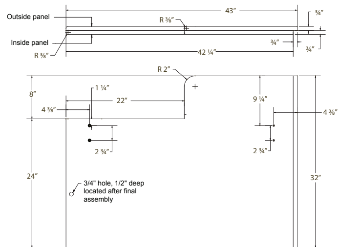
END PANEL
