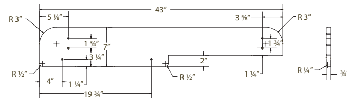
ARM REST
