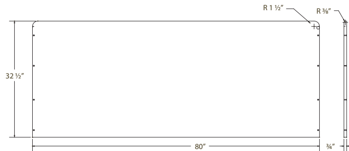
BACK PANEL
