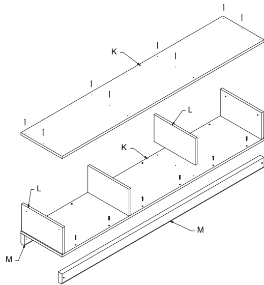
DRAWER UNIT
