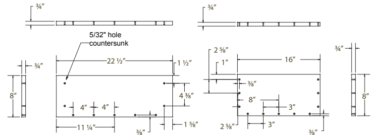
DRAWER SIDE
