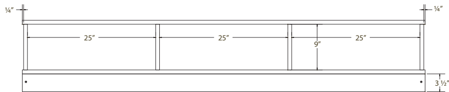
DRAWER UNIT - FRONT VIEW
