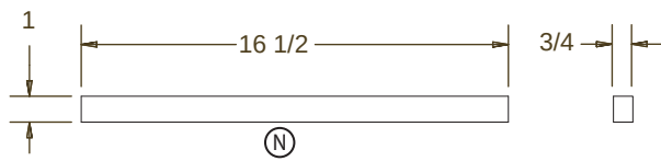
PEG BOARD EDGING (X1)
