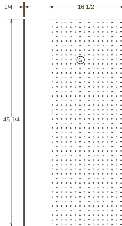
PEG BOARD
