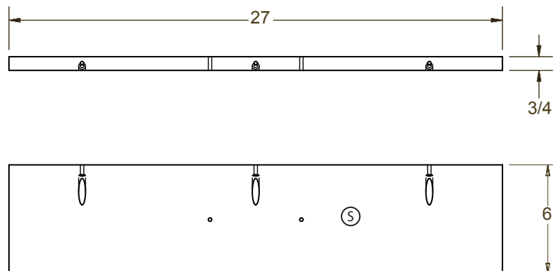
TOP FRONT
