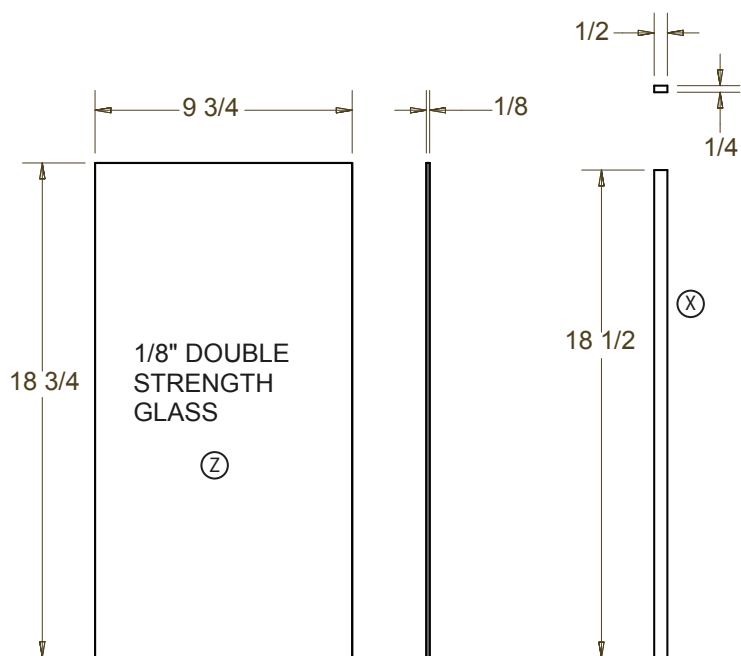
GLASS STOP VERT. (4)
