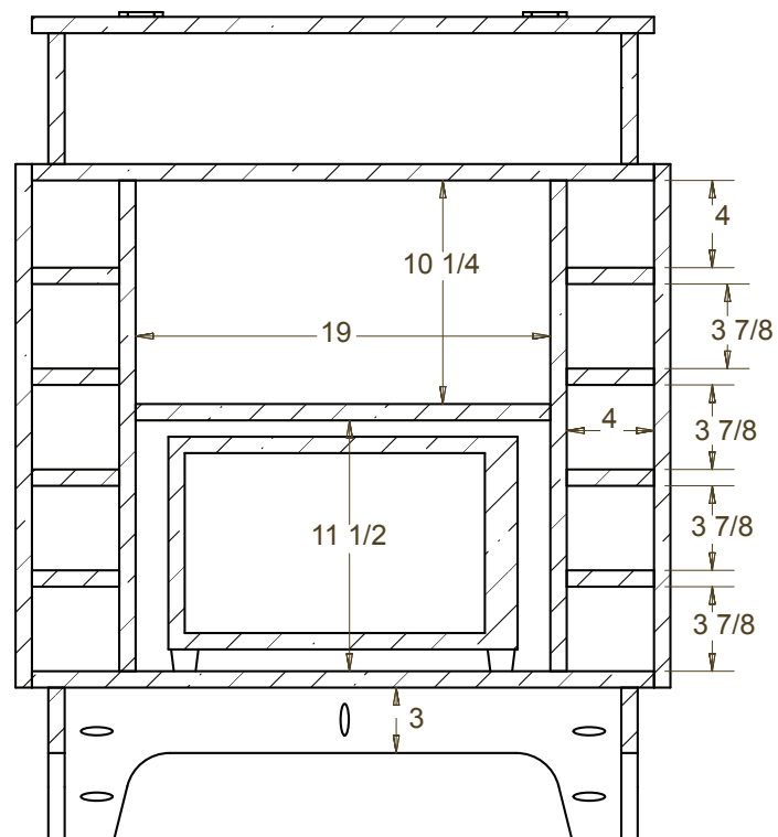
SECTION VIEW
