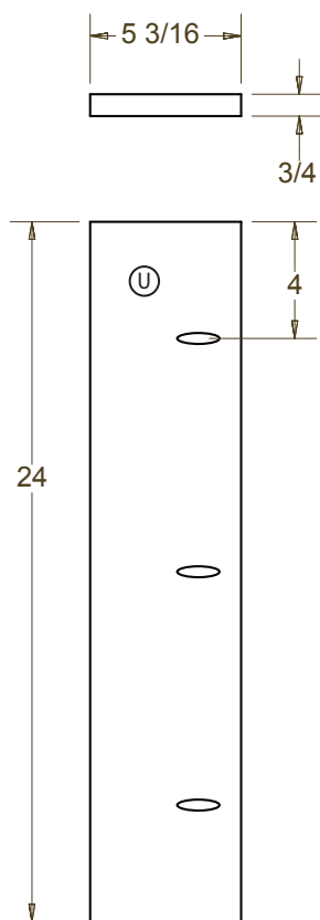
DOOR HINGE BOARD RT
