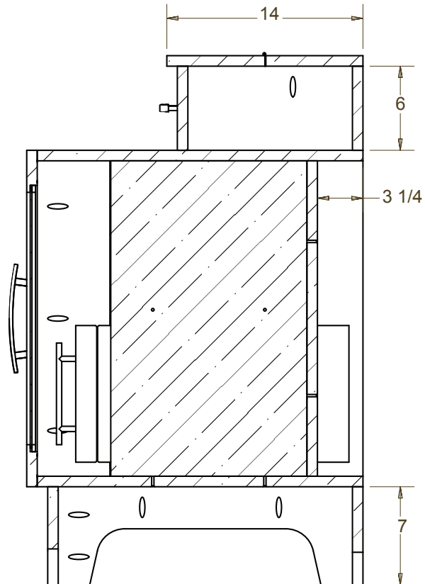
SECTION VIEW
