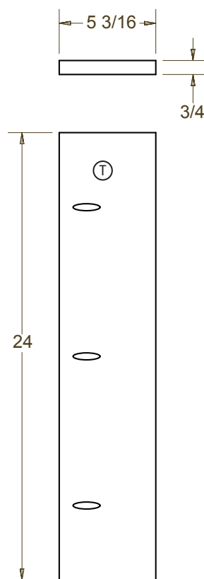
DOOR HINGE BOARD LT
