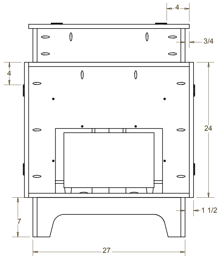
BACK VIEW
