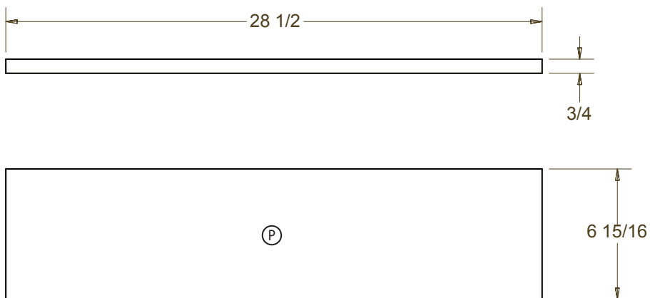
TOP FIXED PANEL
