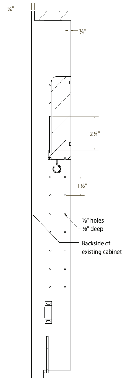
SECTION VIEW
