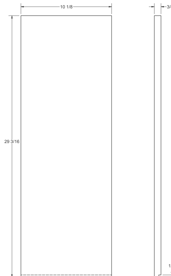
DOOR PANEL (outside face)
