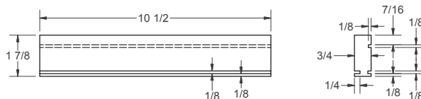
SHELF (top side)
