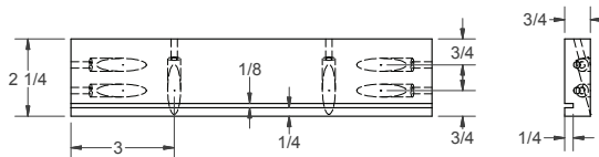
BOTTOM (top side)
