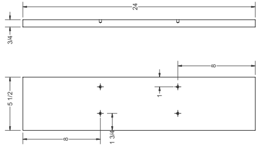
MIRROR WEDGE BACKER (X4)
