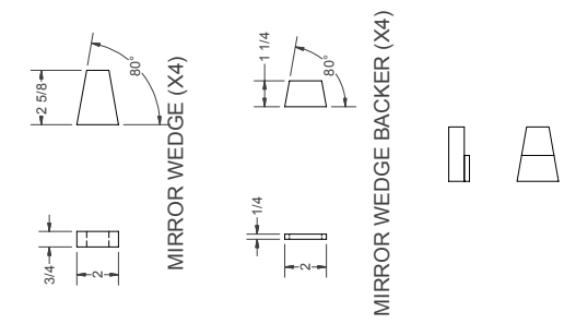
MIRROR WEDGE (X4)
