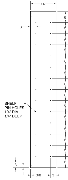
TOWER PANEL
