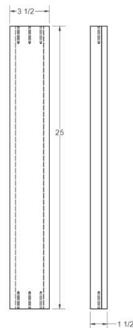
CENTER STRETCHER - C
