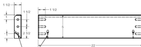
UPPER ARM RAIL - D
