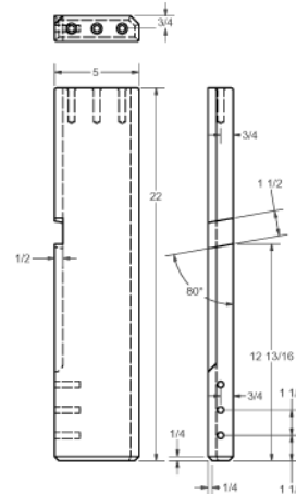
RIGHT FRONT LEG - A
