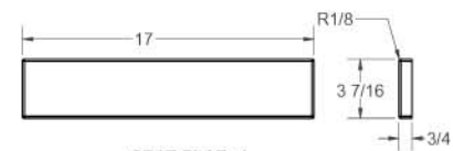
SEAT SLAT - L (5 required)
