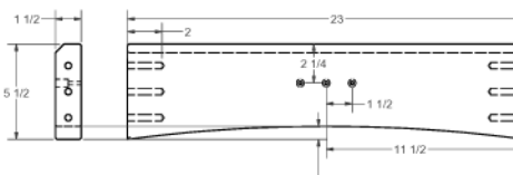
LOWER LEG RAIL - B-2
