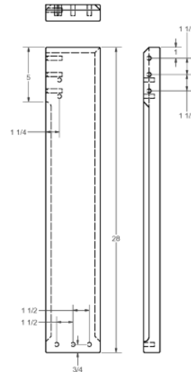
RIGHT ARMREST - C
