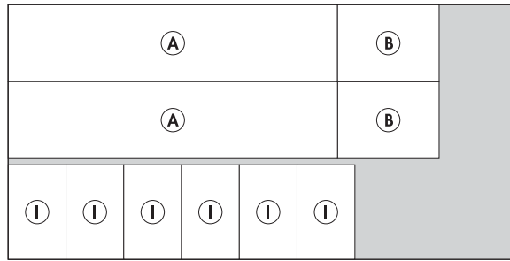
\frac{3}{4} " OAK PLYWOOD - 24" x 48" (QTY: 1)
